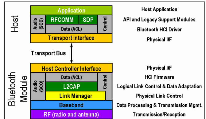
Gambar 8. Bluetooth Protocol Stack
